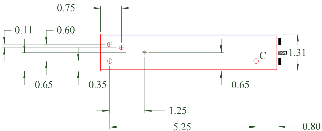
Figure 4-1 Tray Dimensions in inches
