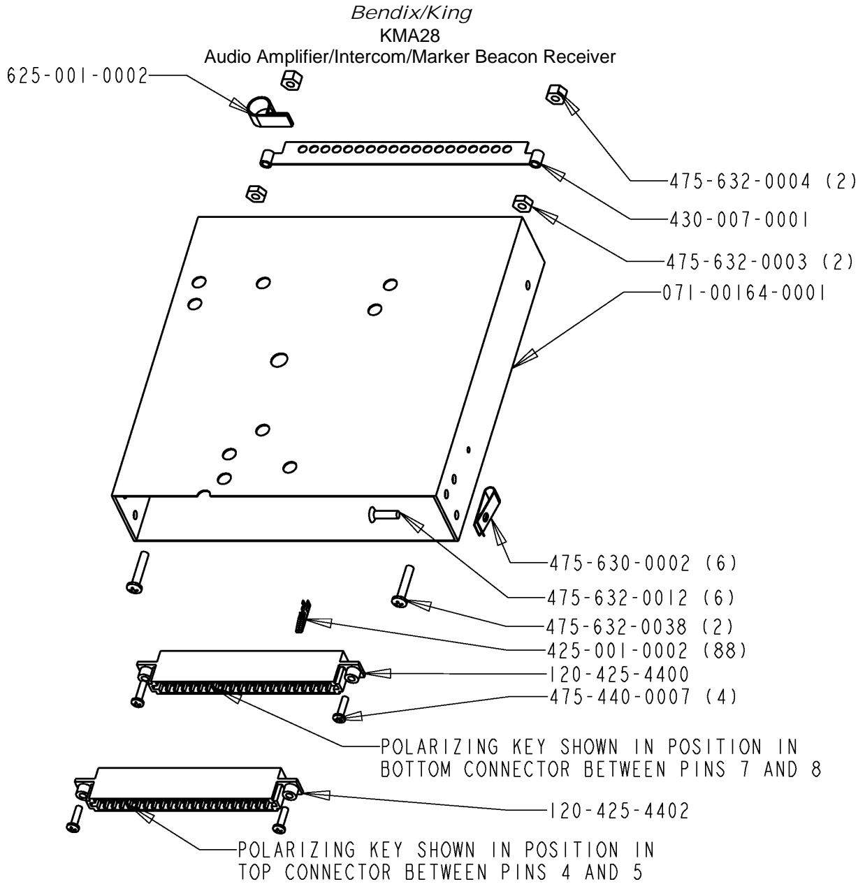
Figure 4-3 Tray Assembly Drawing
