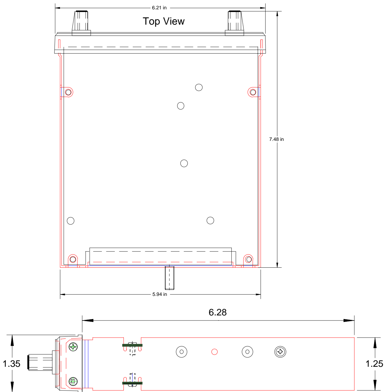
Figure 4-2 Unit External Dimensions in inches
